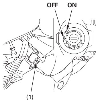
(1) Virtalukko
